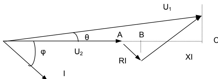
Figura 2. Diagrama vectorial.
